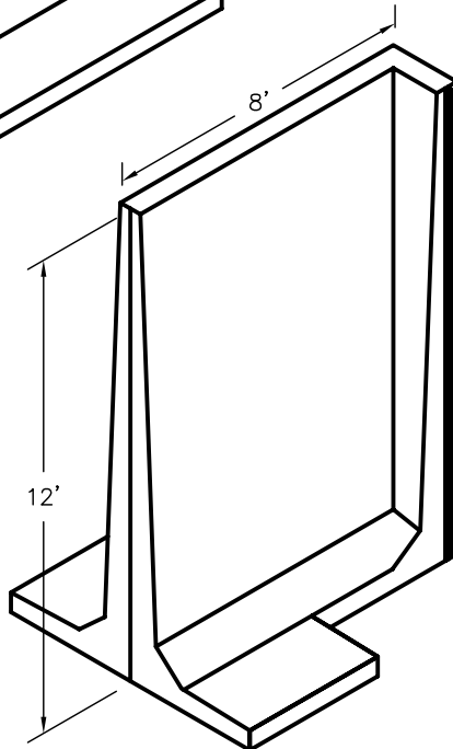
CORNER PANEL
